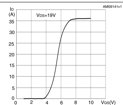
Figure 7. Transfer characteristics
