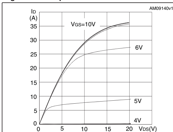
Figure 6. Output characteristics
